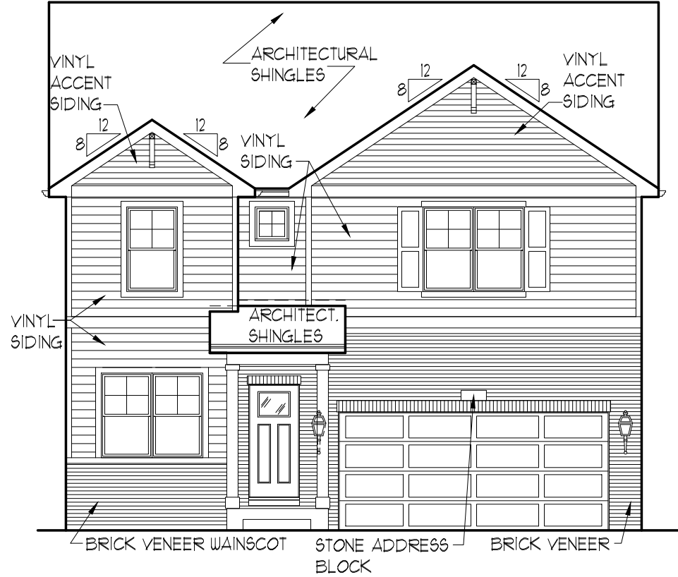
ELEVATION "A4"
