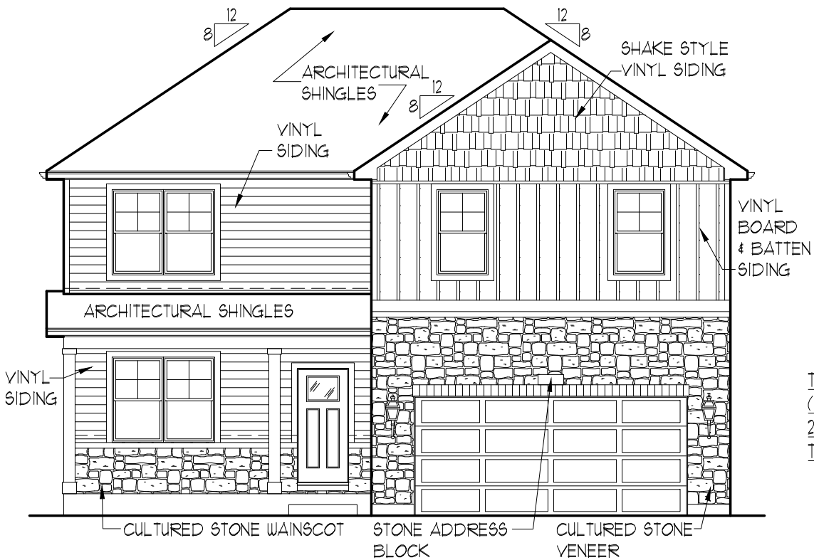
ELEVATION "D5"
