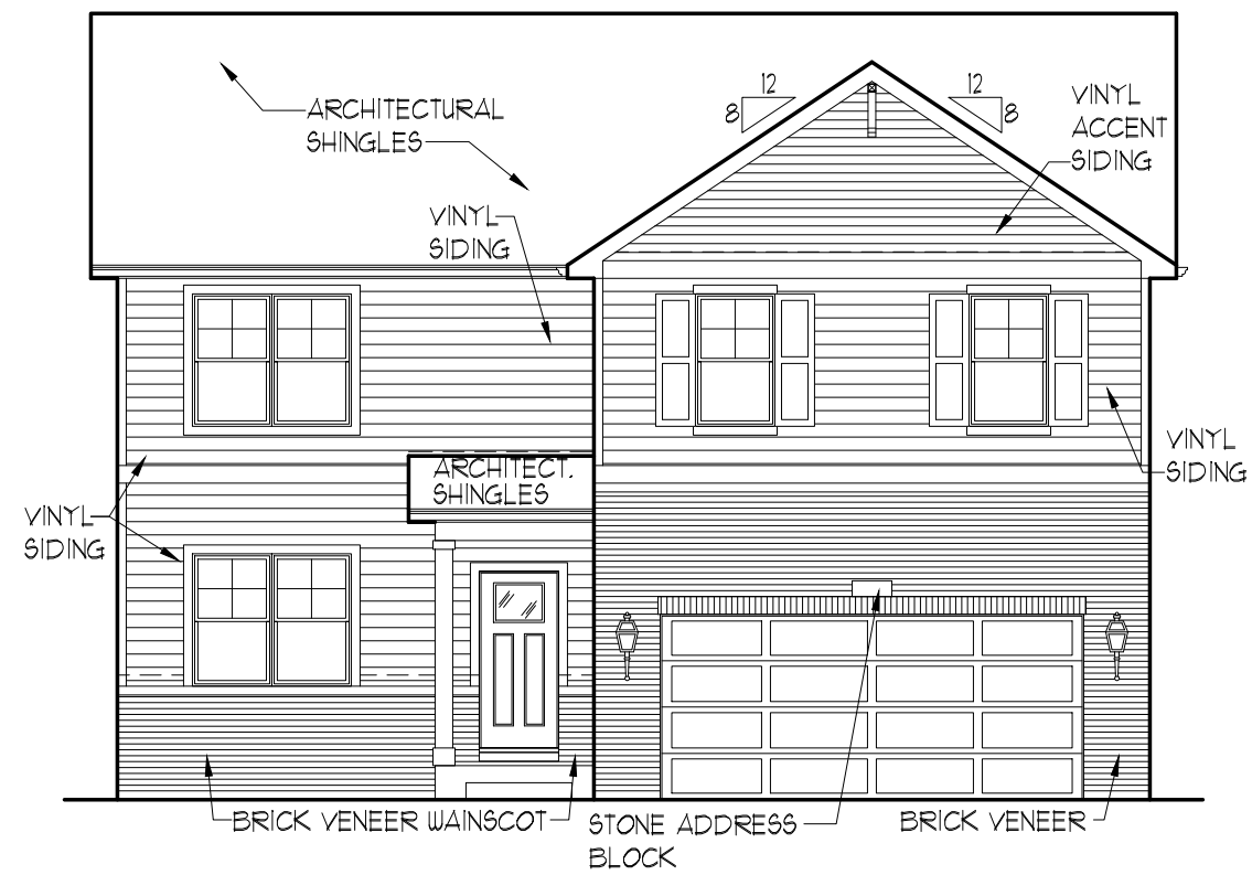
ELEVATION "A4"
