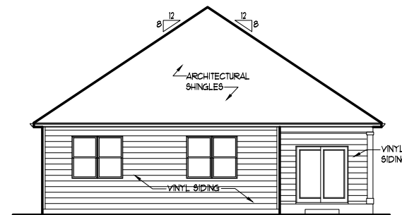
TYPICAL REAR ELEVATION
