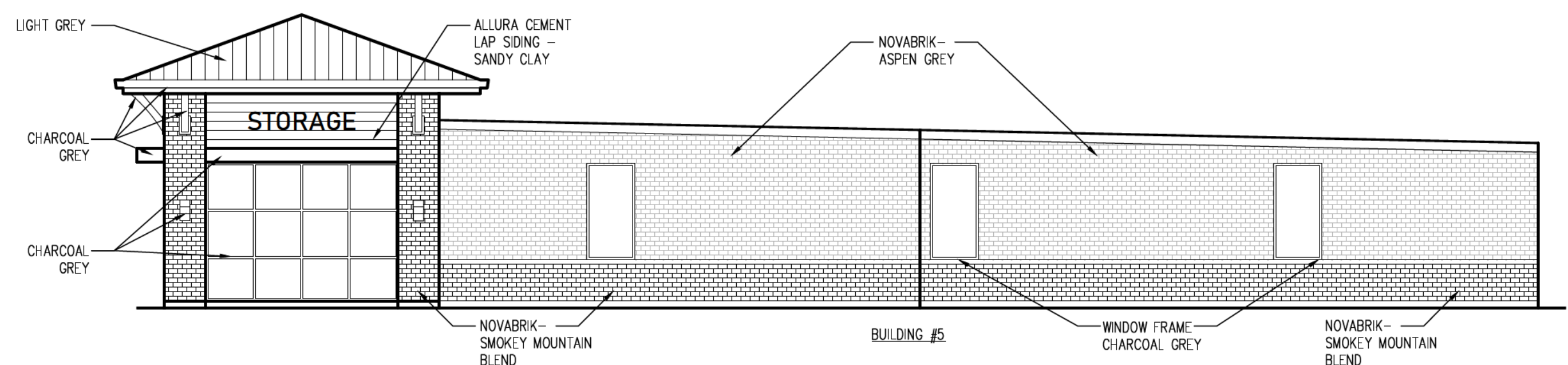
3 NORTHEAST ELEVATION SCALE: 1/8"=1'-0"
