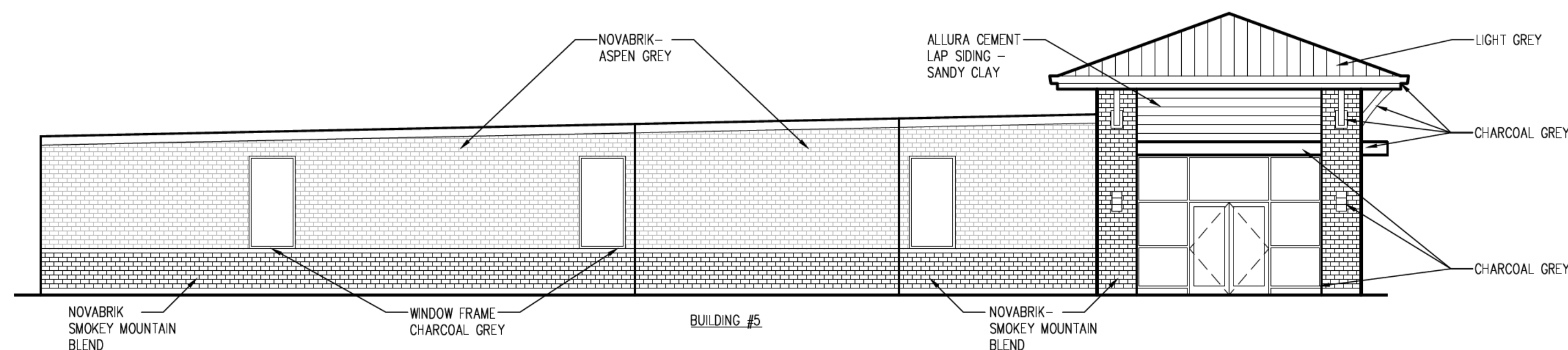
2 SOUTHWEST ELEVATION SCALE: 1/8"=1'-0"
