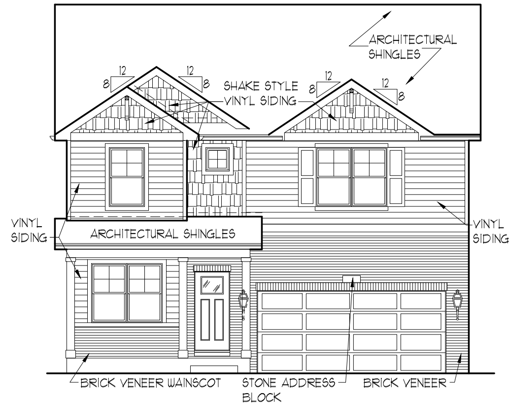
ELEVATION "B4"
